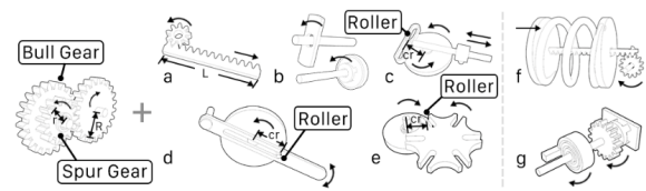
Figure 4: For non-instant motion types, kinetic units combine geartrains (pairs of bull and spur gears) and kinematic transmission mechanisms: (a) rack-and-pinions, (b) axles or revolute joints, (c) Scotch yokes, (d) crank-and-slotted-levers, and (e) Geneva drives. Helical springs engage with gears through (f) rack-and-pinions and (g) spiral springs are co-axial with gears for driving the geartrain.
