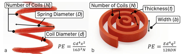
Figure 2: Spring energy source and related parameters: (a) helical spring and (b) spiral spring. Material-related parameters are used for calculating the potential energy in springs: Shear modulus G for helical springs and Young’s modulus E for spiral springs.
