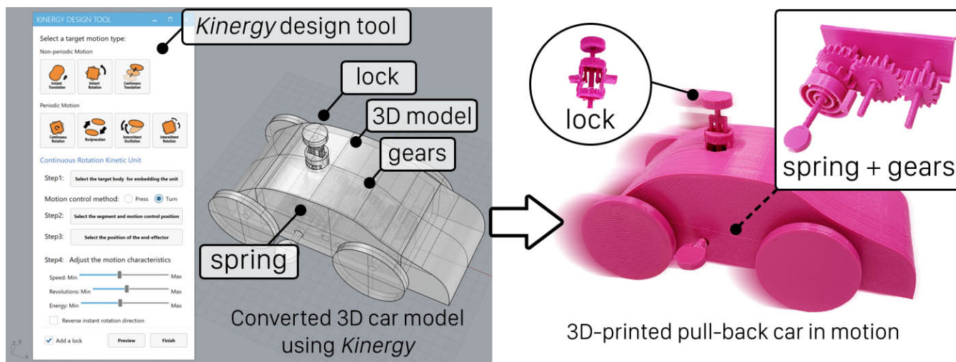
Figure 1: We introduce Kinergy , an interactive design tool to rapidly create 3D printable energy-powered motion. Above, we show a 3D-printed pull-back car created with Kinergy : the static car model is converted into a motion-enabled model with an auto-generated and embedded spring, a spring lock, and a set of gears (left). All the parts in the converted 3D car model are printed in place with a commercial 3D printer and the printed car is ready to move without post-print part assembly (right).
